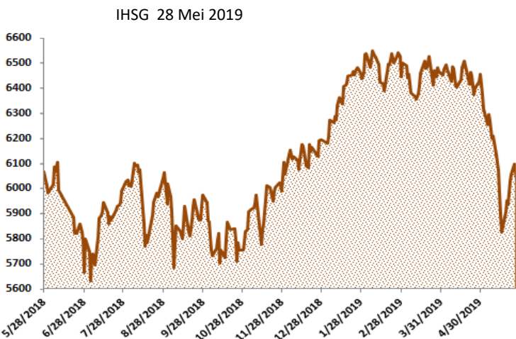
IHSG Statistics
