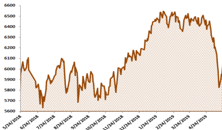
IHSG Statistics
