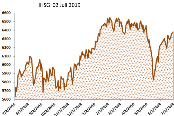
IHSG Statistics
